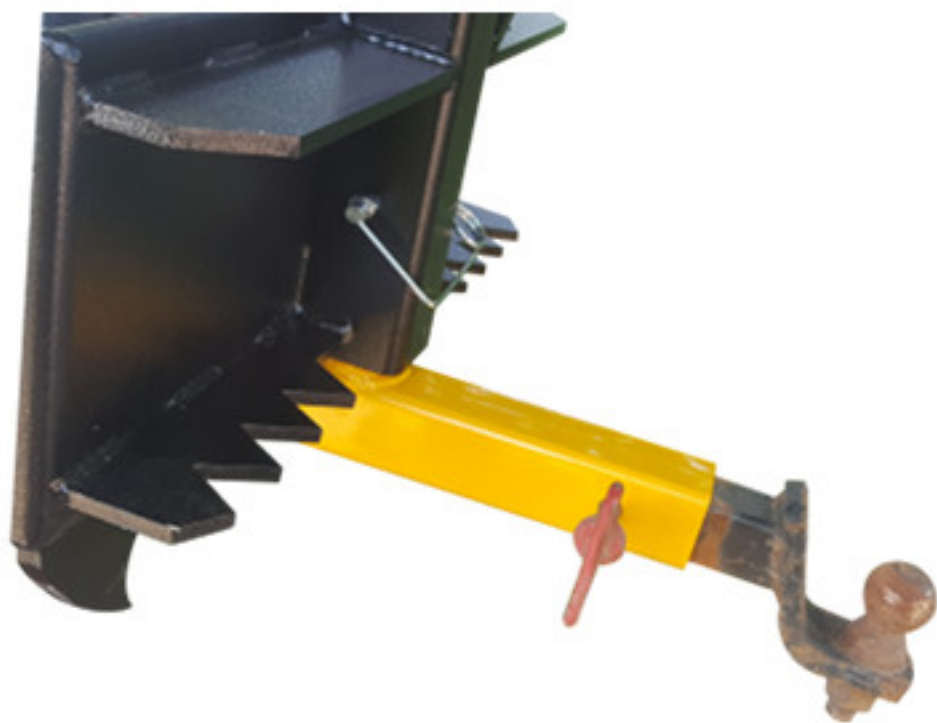
Receiver Hitch to move your chipper
